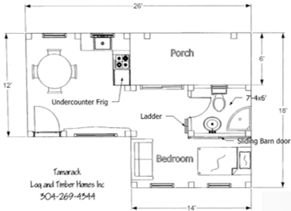
Main Floor
